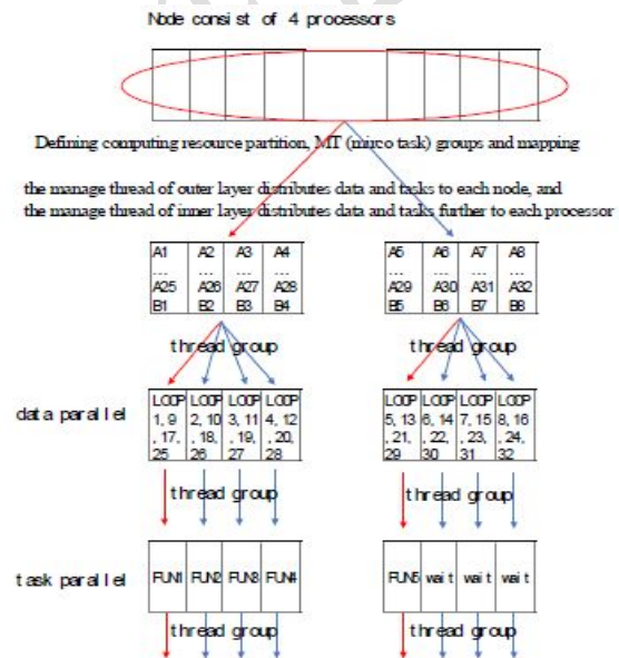
Figure 4: Fine Grain Execution Model
