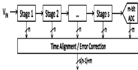
Figure 2: Pipelined ADC Block Diagram
