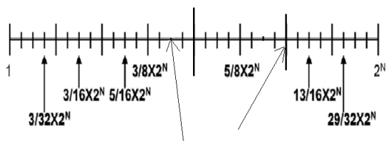
Figure 7: Ideal Case of Transition Edge
