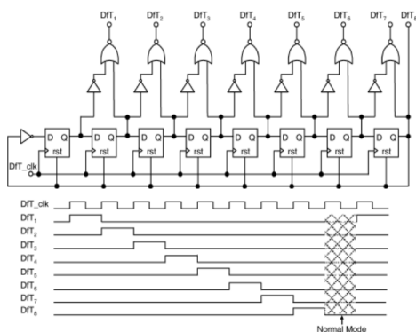
Figure 8: DEC Logic Diagram
